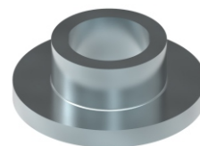
⑯ 翻边衬套*4 \phi 6.2 \times \phi 8.4 \times 3.5 + \phi 14 \times 1.5 1274100-057095
