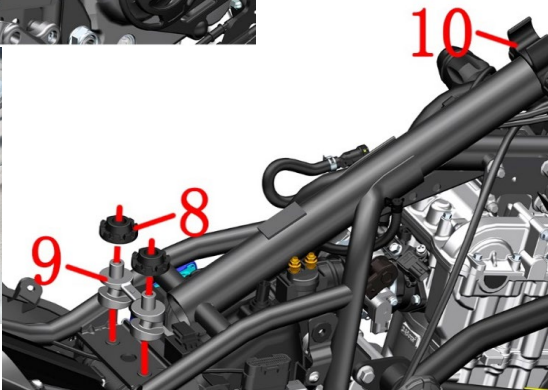
Fuel tank lock plug
